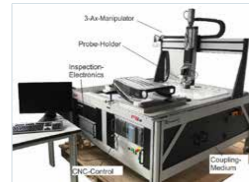
Construction and elements of the online-monitoring system at Fraunhofer ICT
