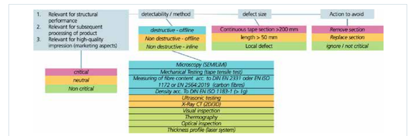
Classification of defects of UD tape products
