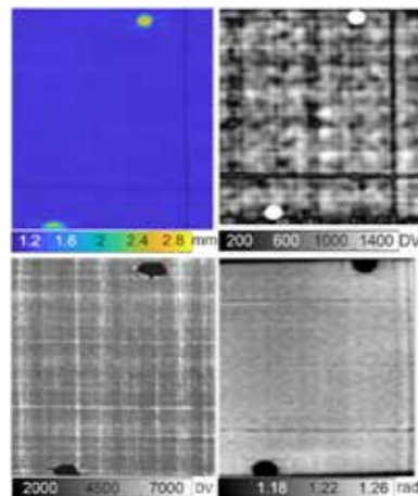
Results of laminate with gaps.
